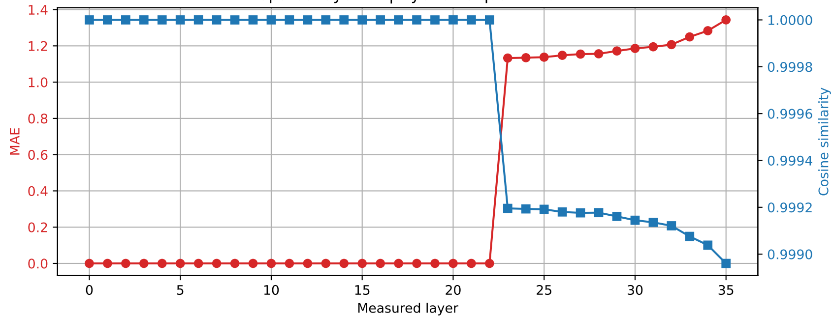
Qwen2.5-3B | Prompt 2 Spared layer 22 | Hybrid vs quantized
