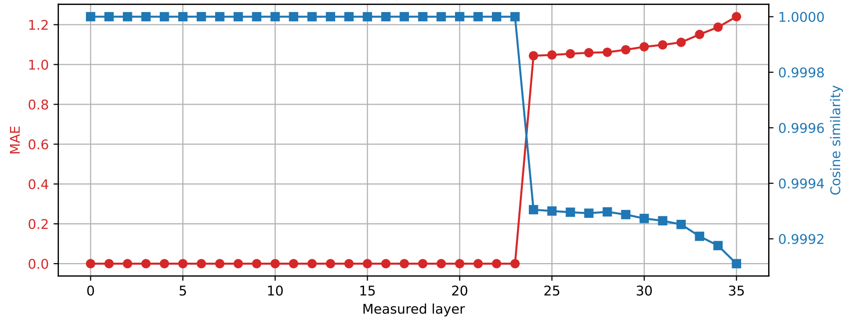
Qwen2.5-3B | Prompt 2 Spared layer 23 | Hybrid vs quantized
