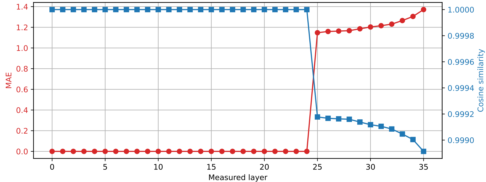
Qwen2.5-3B | Prompt 2 Spared layer 24 | Hybrid vs quantized
