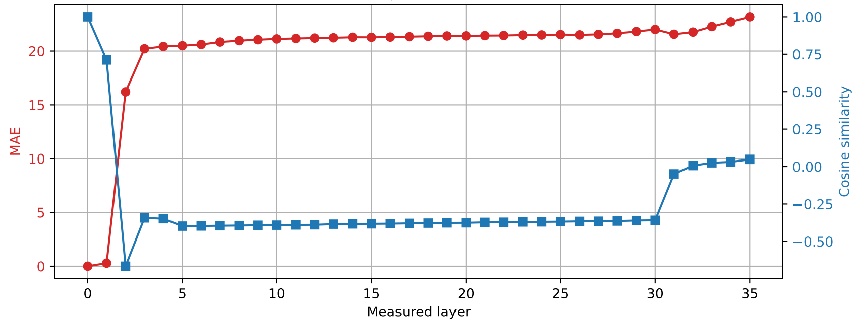
Qwen2.5-3B | Prompt 2 Spared layer 25 | Hybrid vs unquantized
