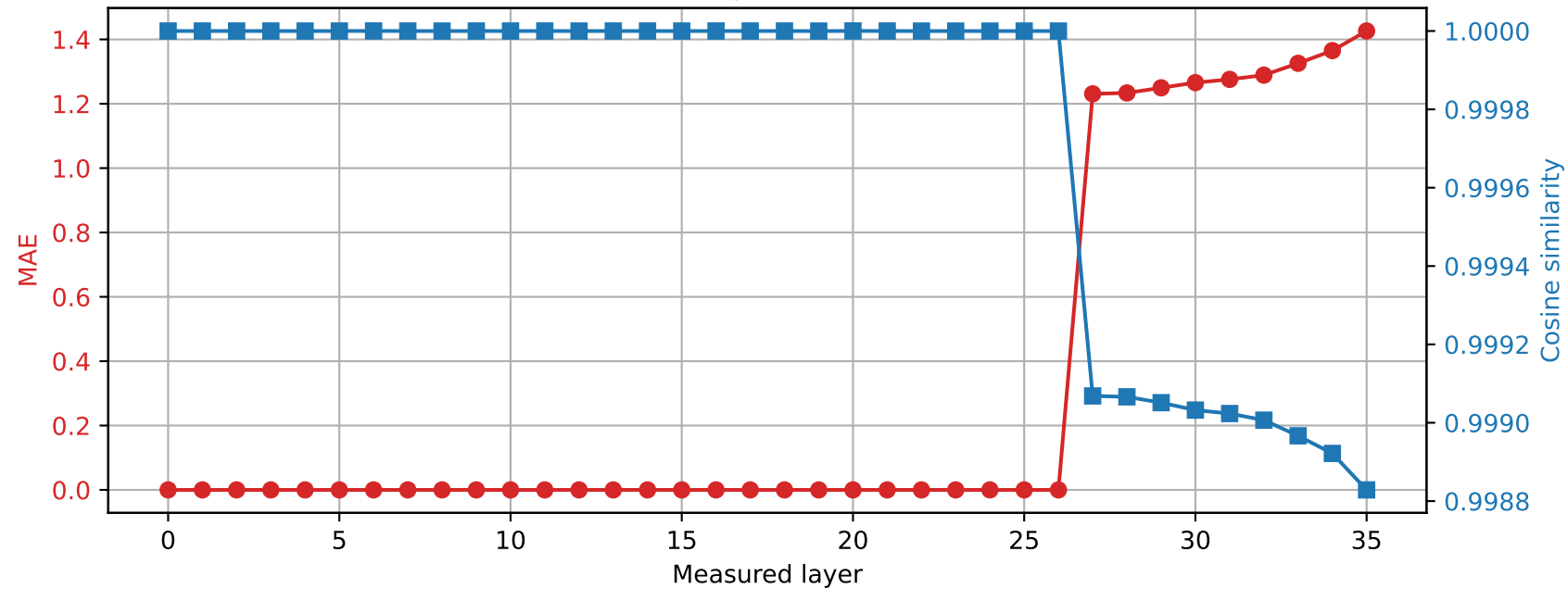
Qwen2.5-3B | Prompt 2 Spared layer 26 | Hybrid vs quantized
