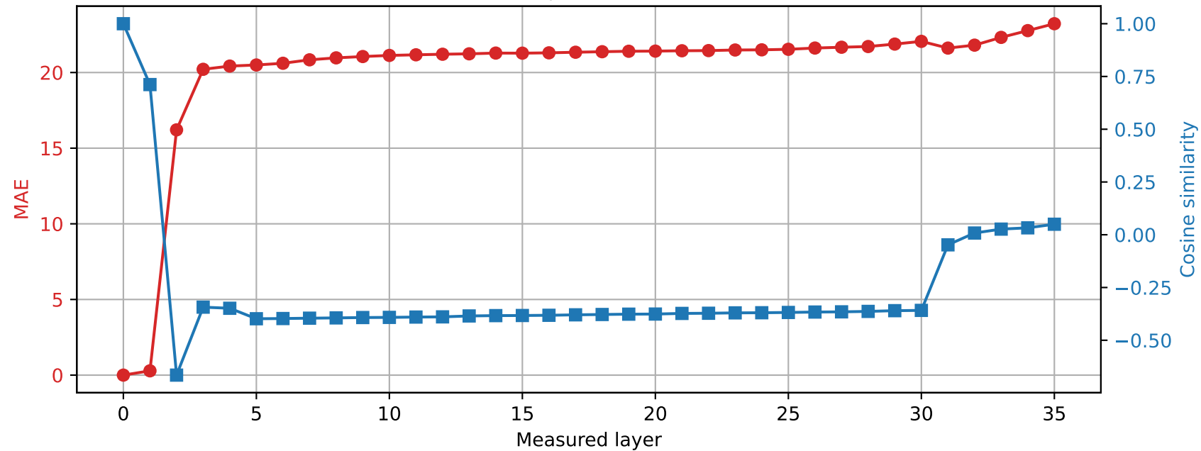
Qwen2.5-3B | Prompt 2 Spared layer 27 | Hybrid vs unquantized
