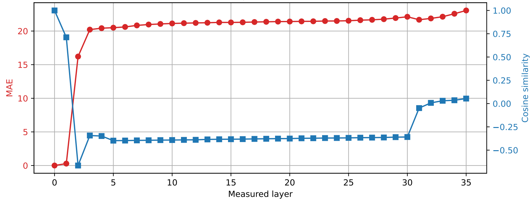
Qwen2.5-3B | Prompt 2 Spared layer 32 | Hybrid vs unquantized
