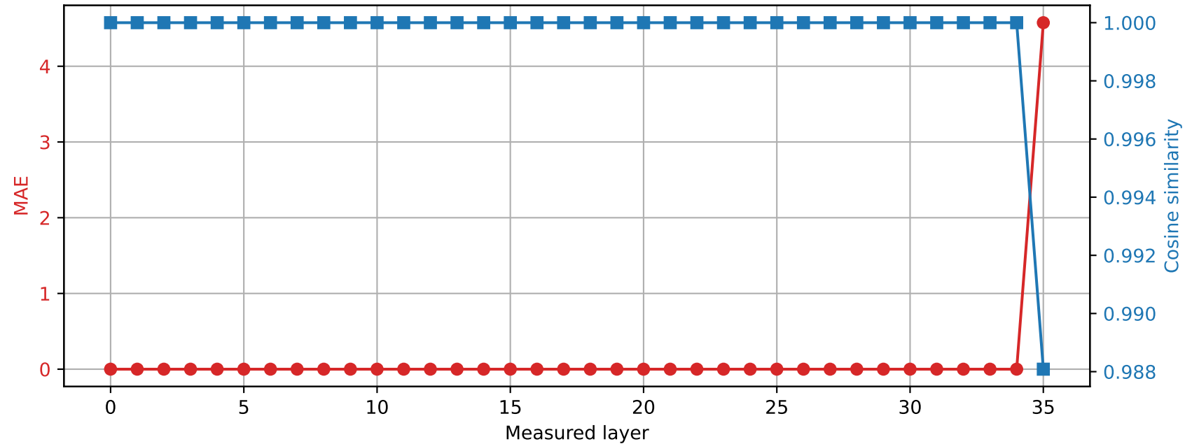
Qwen2.5-3B | Prompt 2 Spared layer 34 | Hybrid vs quantized
