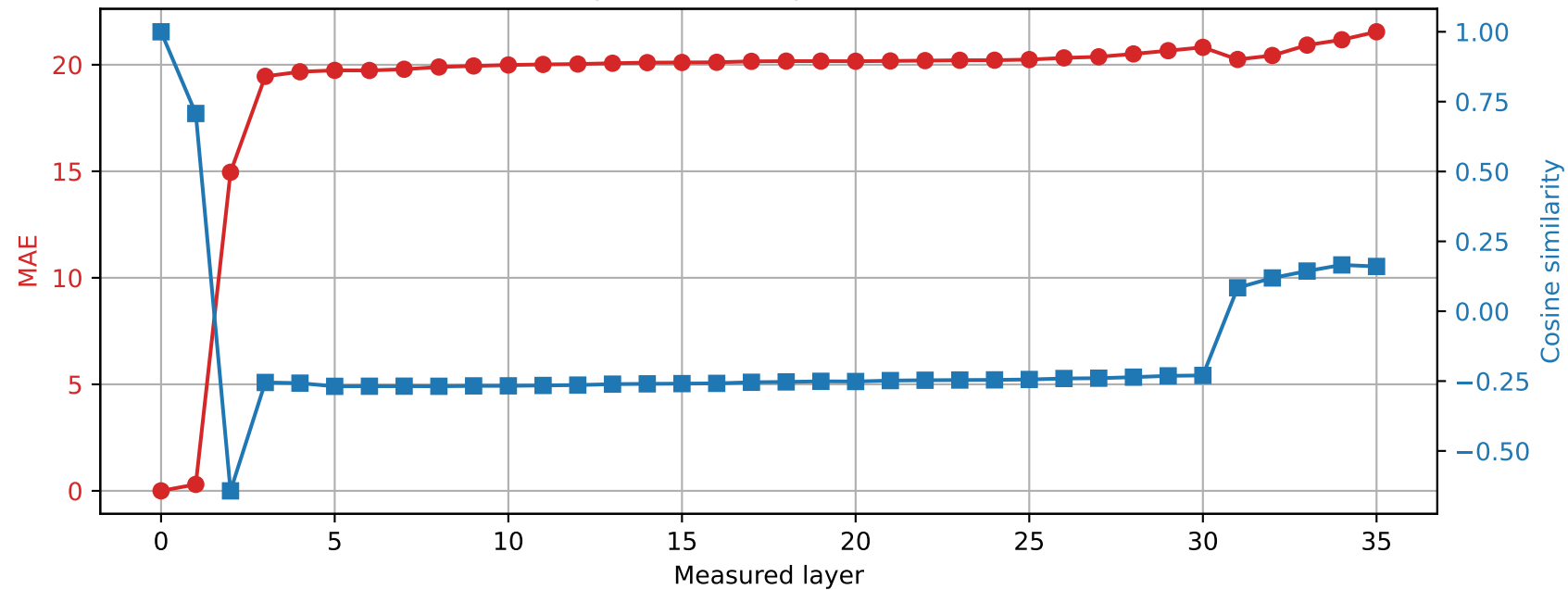
Qwen2.5-3B | Prompt 3 Unquantized vs quantized int4
