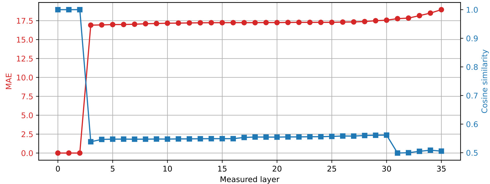
Qwen2.5-3B | Prompt 3 Spared layer 2 | Hybrid vs quantized
