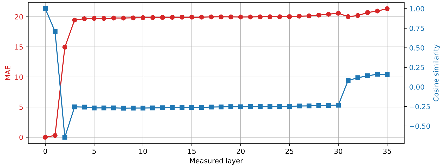
Qwen2.5-3B | Prompt 3 Spared layer 7 | Hybrid vs unquantized
