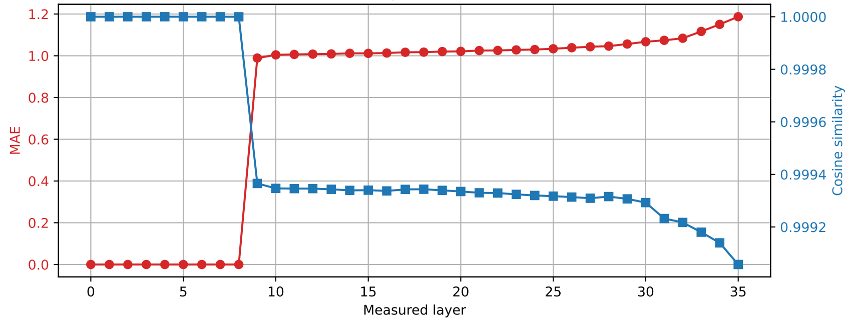
Qwen2.5-3B | Prompt 3 Spared layer 8 | Hybrid vs quantized
