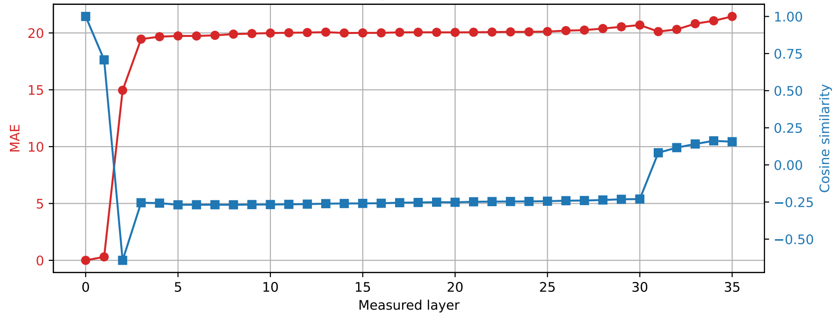
Qwen2.5-3B | Prompt 3 Spared layer 13 | Hybrid vs unquantized
