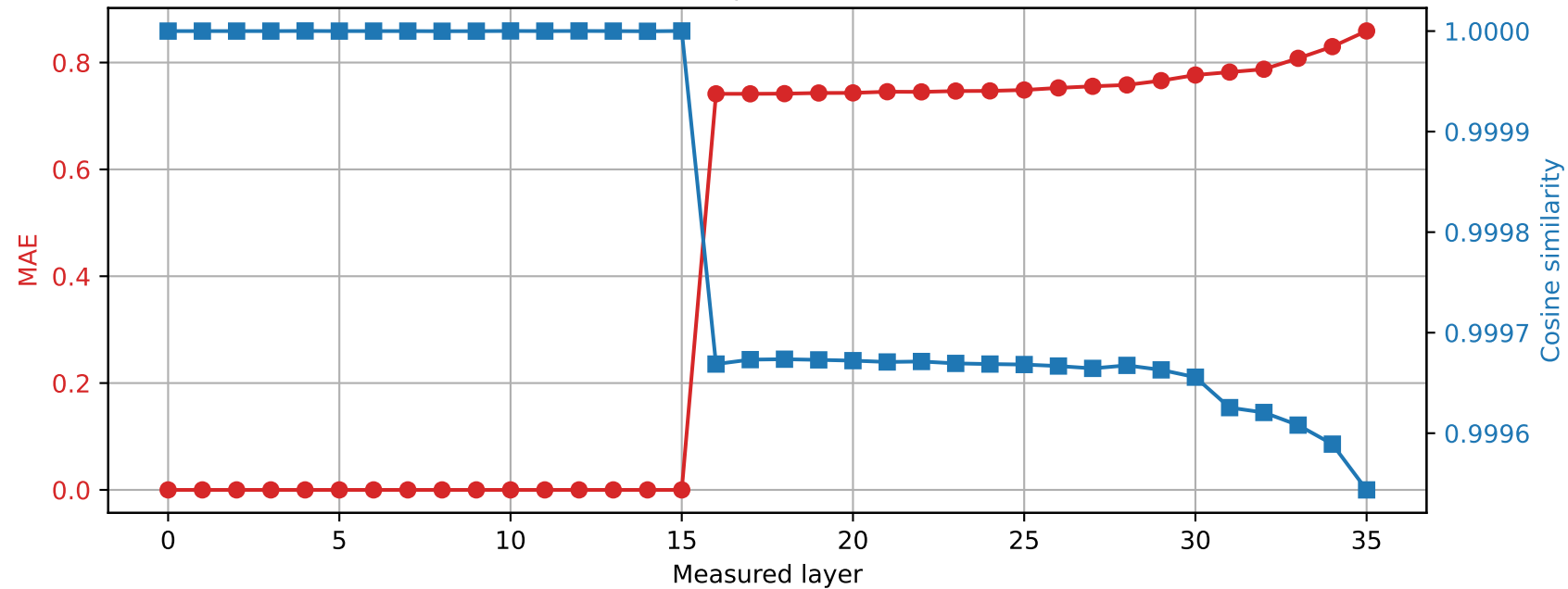
Qwen2.5-3B | Prompt 3 Spared layer 15 | Hybrid vs quantized
