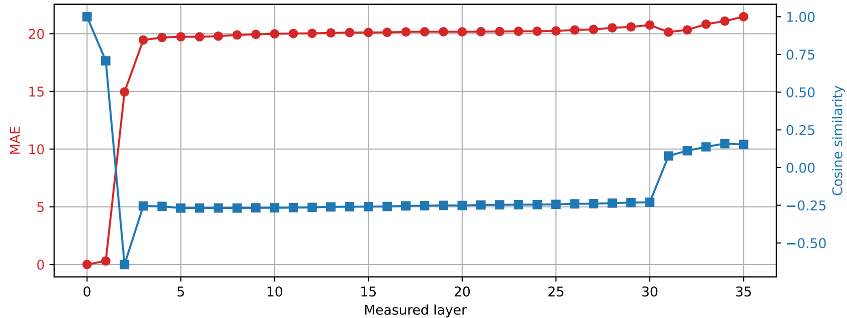
Qwen2.5-3B | Prompt 3 Spared layer 28 | Hybrid vs unquantized
