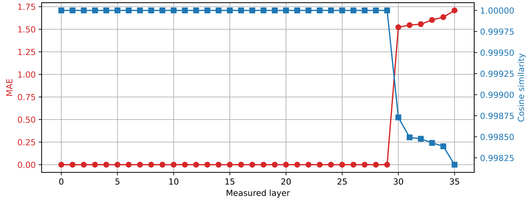
Qwen2.5-3B | Prompt 3 Spared layer 29 | Hybrid vs quantized
