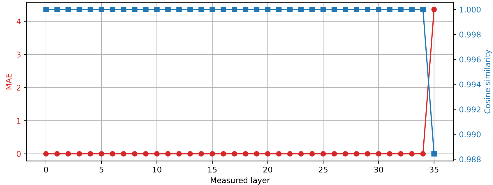
Qwen2.5-3B | Prompt 3 Spared layer 34 | Hybrid vs quantized
