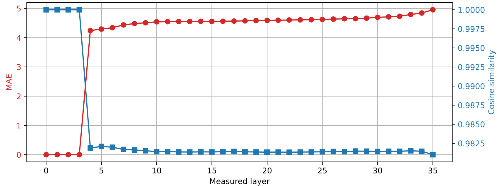
Qwen2.5-3B | Prompt 4 Spared layer 3 | Hybrid vs quantized
