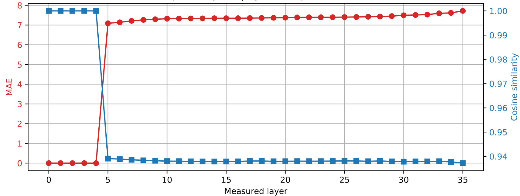
Qwen2.5-3B | Prompt 4 Spared layer 4 | Hybrid vs quantized
