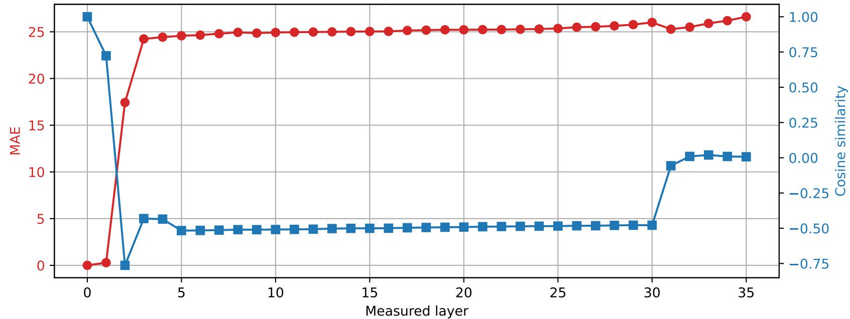
Qwen2.5-3B | Prompt 4 Spared layer 8 | Hybrid vs unquantized
