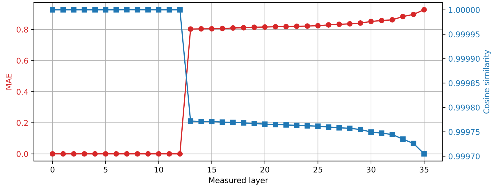
Qwen2.5-3B | Prompt 4 Spared layer 12 | Hybrid vs quantized
