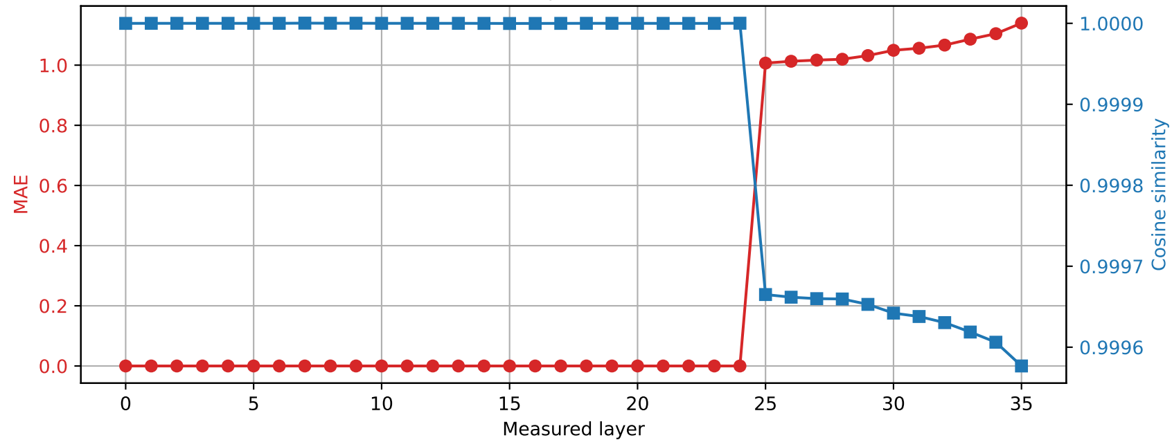
Qwen2.5-3B | Prompt 4 Spared layer 24 | Hybrid vs quantized
