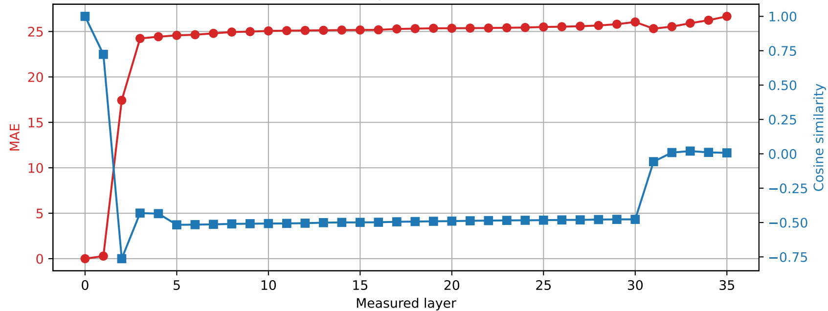
Qwen2.5-3B | Prompt 4 Spared layer 25 | Hybrid vs unquantized
