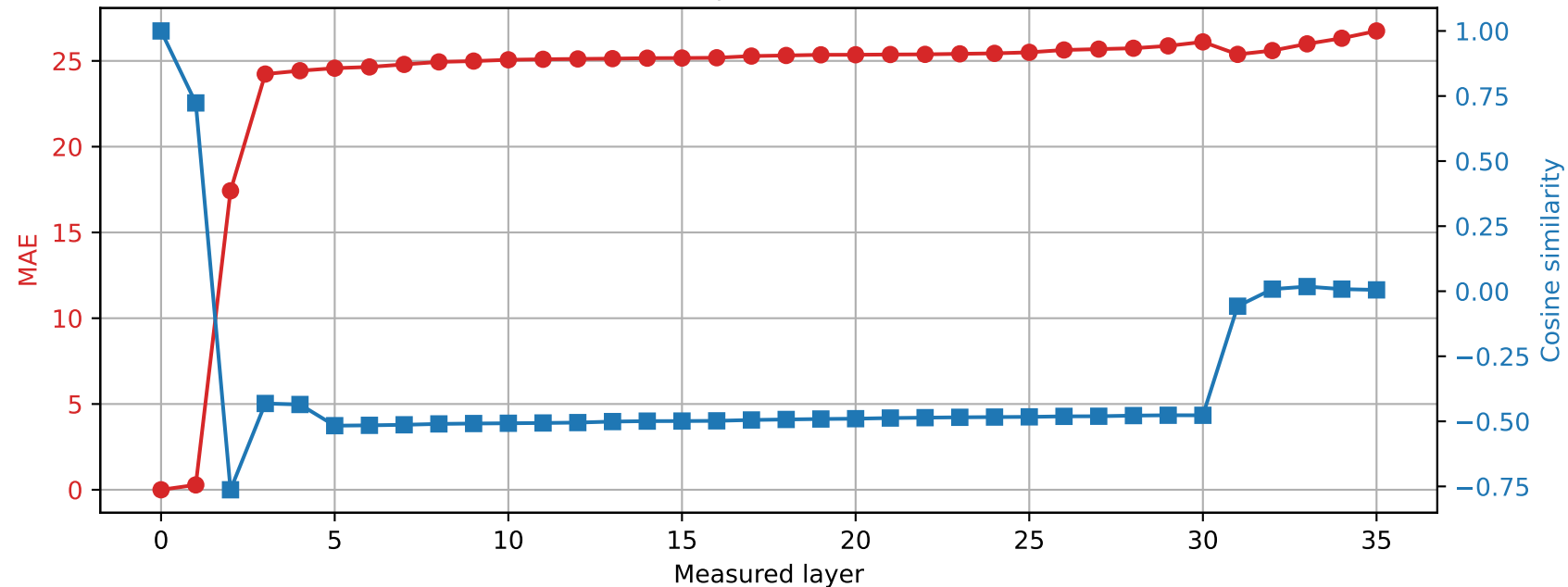
Qwen2.5-3B | Prompt 4 Spared layer 27 | Hybrid vs unquantized
