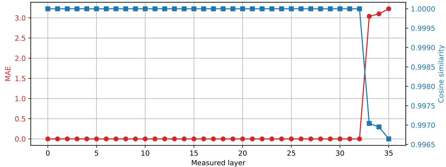
Qwen2.5-3B | Prompt 4 Spared layer 32 | Hybrid vs quantized
