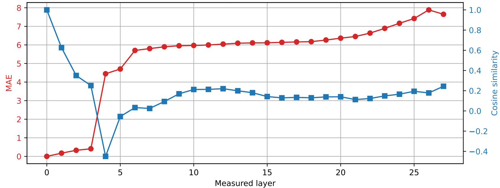
Qwen2.5-7B-Instruct | Prompt 0 Spared layer 5 | Hybrid vs unquantized
