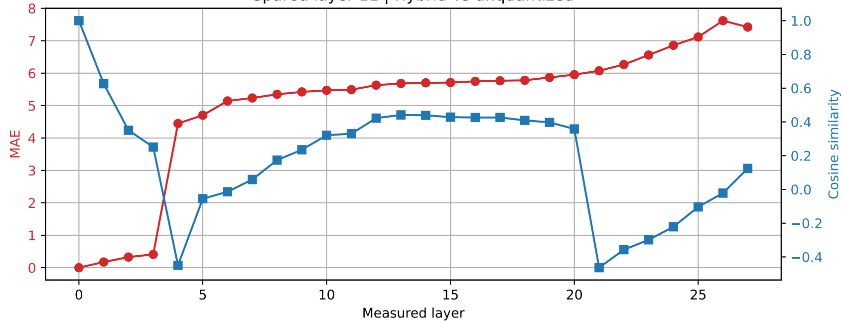
Qwen2.5-7B-Instruct | Prompt 0 Spared layer 11 | Hybrid vs unquantized
