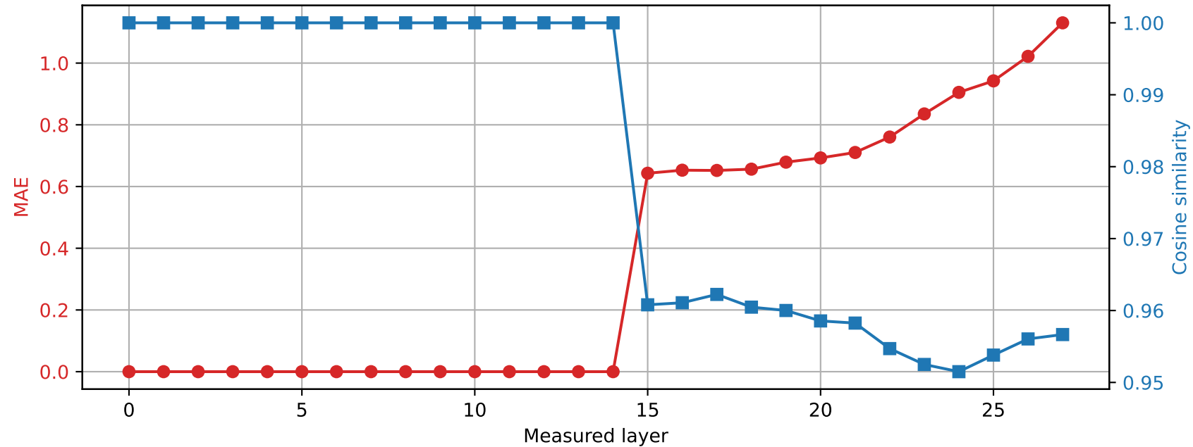
Qwen2.5-7B-Instruct | Prompt 0 Spared layer 14 | Hybrid vs quantized
