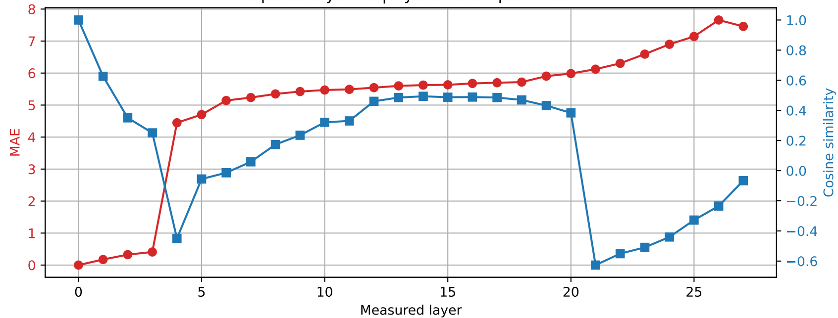
Qwen2.5-7B-Instruct | Prompt 0 Spared layer 18 | Hybrid vs unquantized
