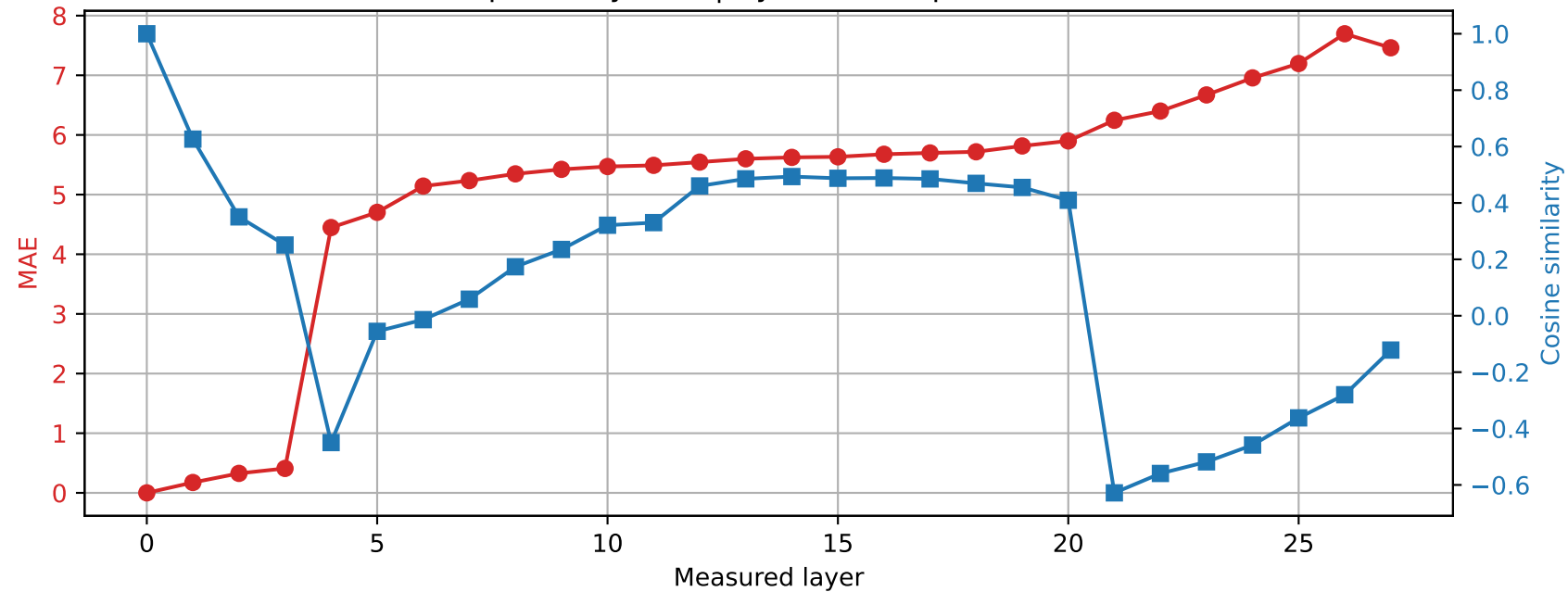
Qwen2.5-7B-Instruct | Prompt 0 Spared layer 20 | Hybrid vs unquantized
