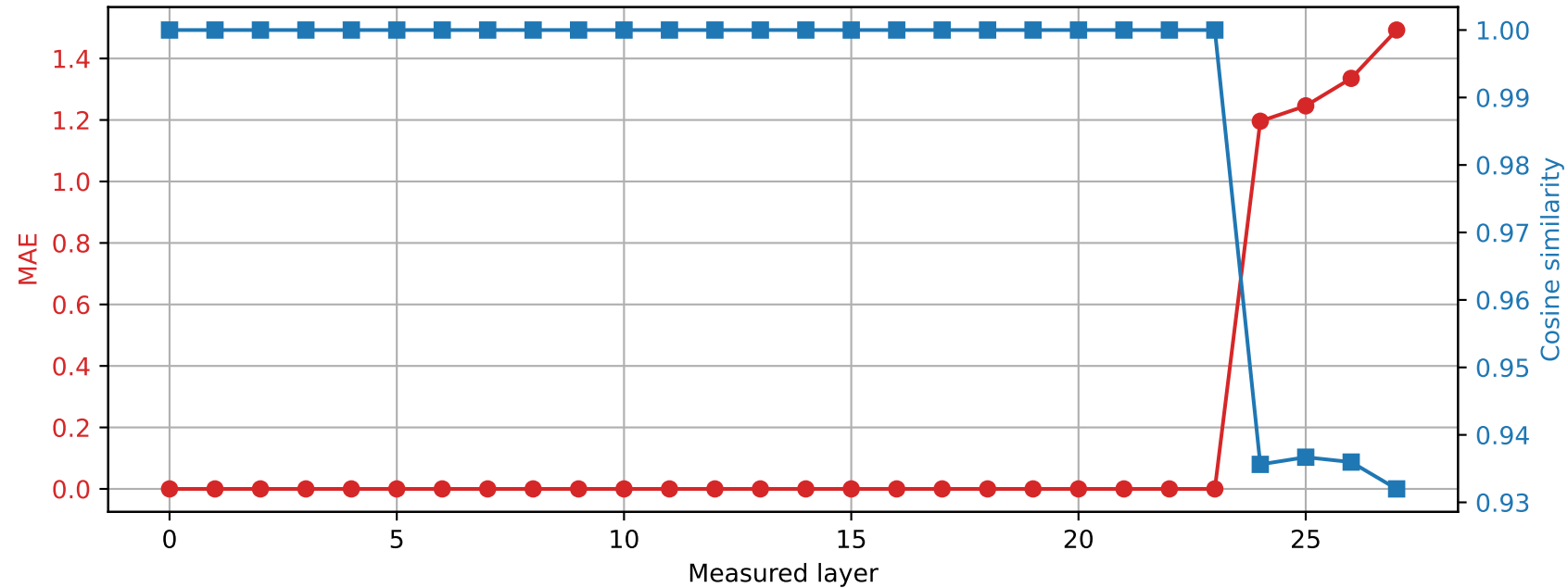
Qwen2.5-7B-Instruct | Prompt 0 Spared layer 23 | Hybrid vs quantized
