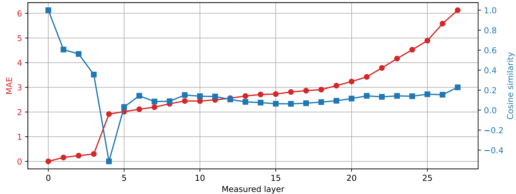
Qwen2.5-7B-Instruct | Prompt 1 Spared layer 3 | Hybrid vs unquantized
