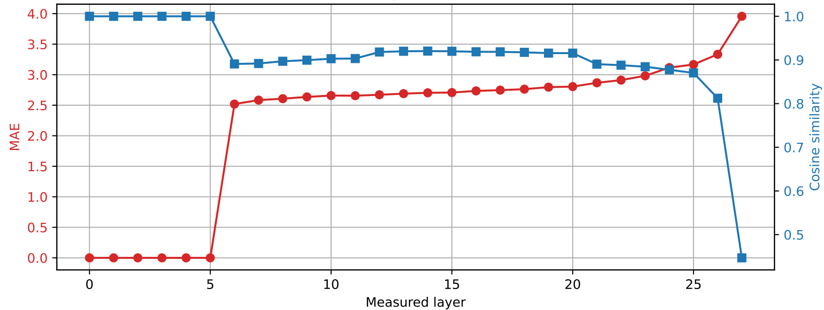
Qwen2.5-7B-Instruct | Prompt 1 Spared layer 5 | Hybrid vs quantized
