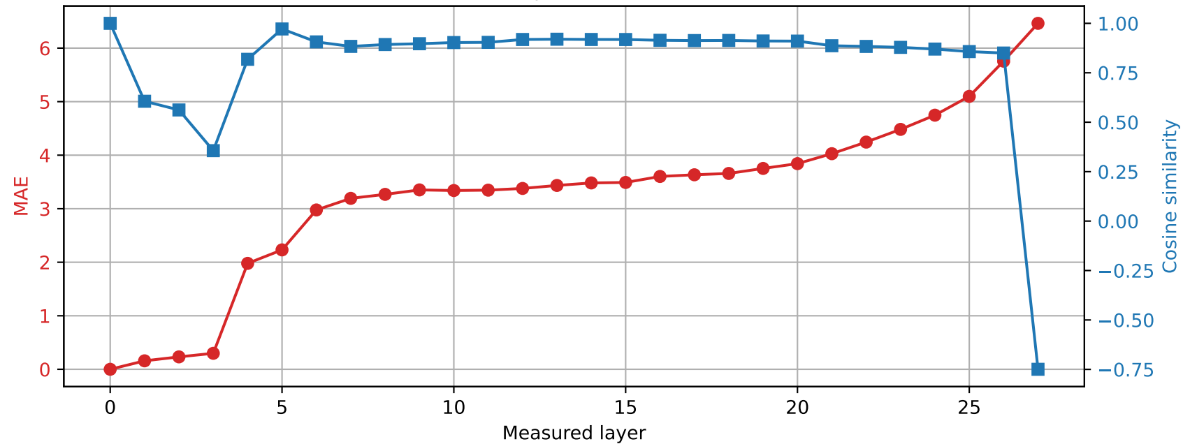
Qwen2.5-7B-Instruct | Prompt 1 Spared layer 15 | Hybrid vs unquantized
