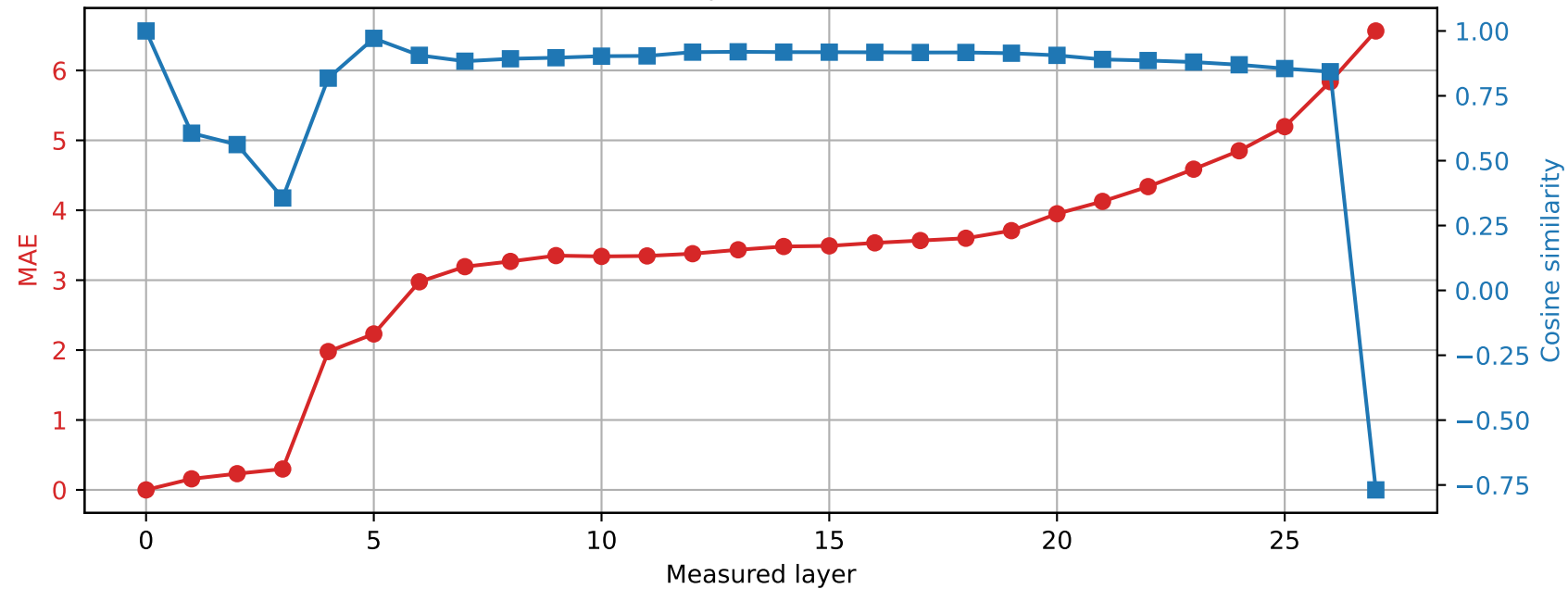
Qwen2.5-7B-Instruct | Prompt 1 Spared layer 19 | Hybrid vs unquantized
