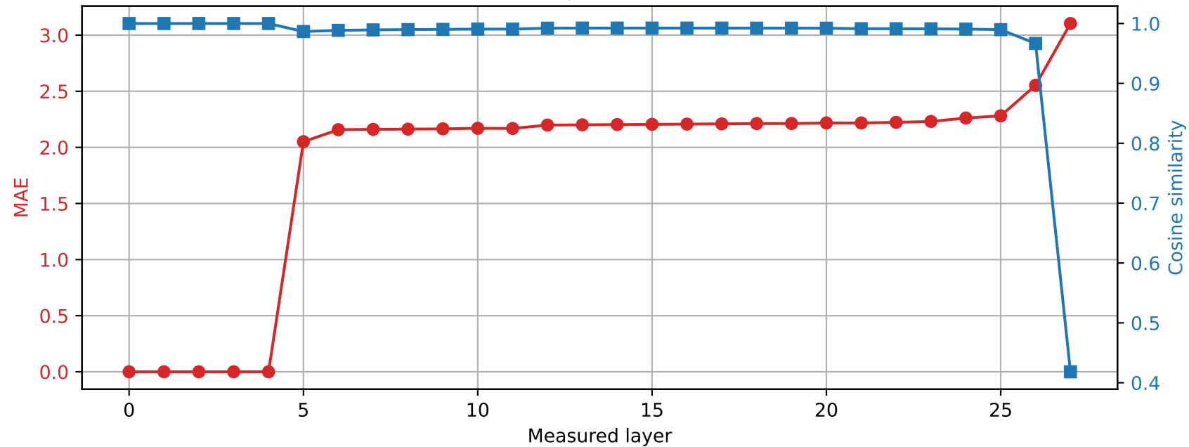
Qwen2.5-7B-Instruct | Prompt 2 Spared layer 4 | Hybrid vs quantized
