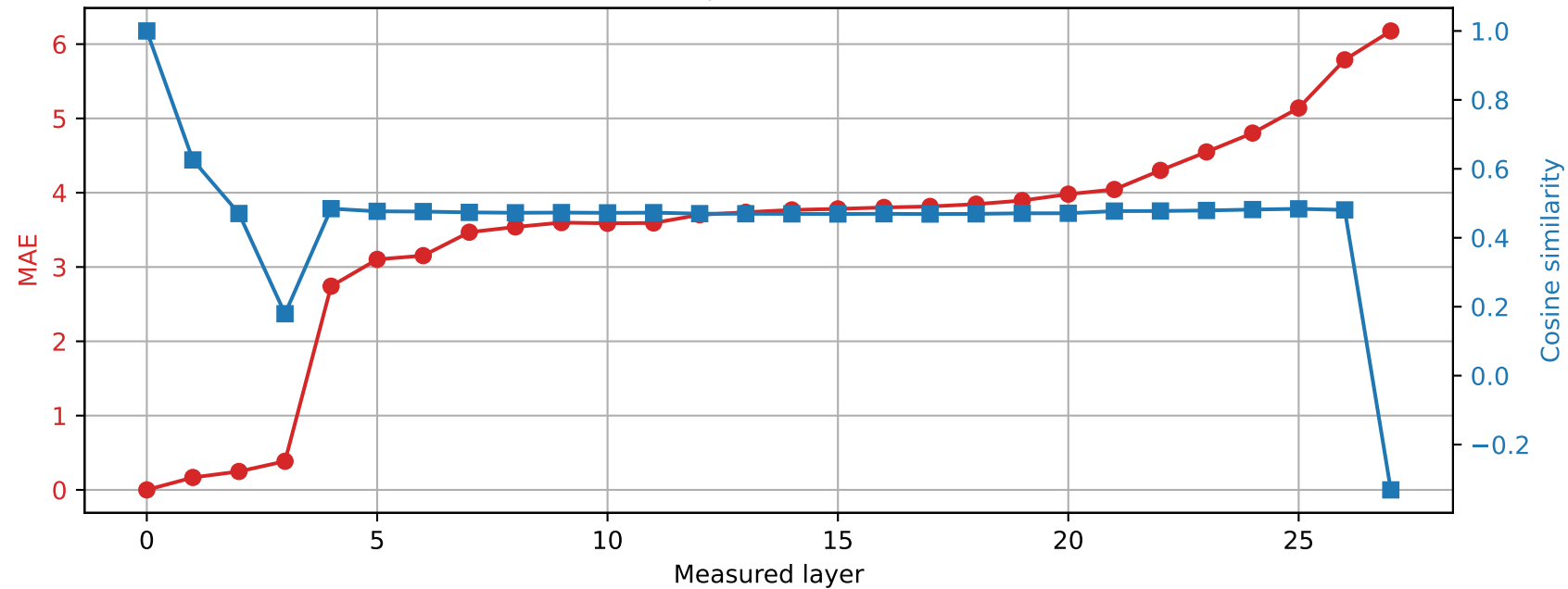
Qwen2.5-7B-Instruct | Prompt 2 Spared layer 6 | Hybrid vs unquantized
