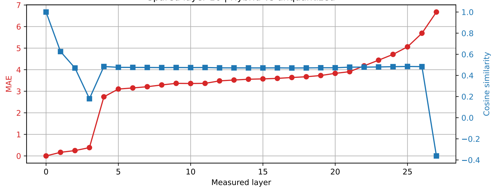
Qwen2.5-7B-Instruct | Prompt 2 Spared layer 16 | Hybrid vs unquantized
