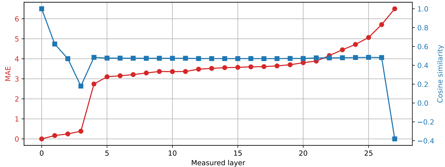
Qwen2.5-7B-Instruct | Prompt 2 Spared layer 22 | Hybrid vs unquantized
