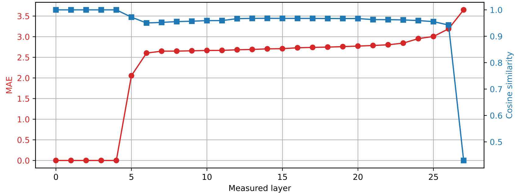
Qwen2.5-7B-Instruct | Prompt 3 Spared layer 4 | Hybrid vs quantized
