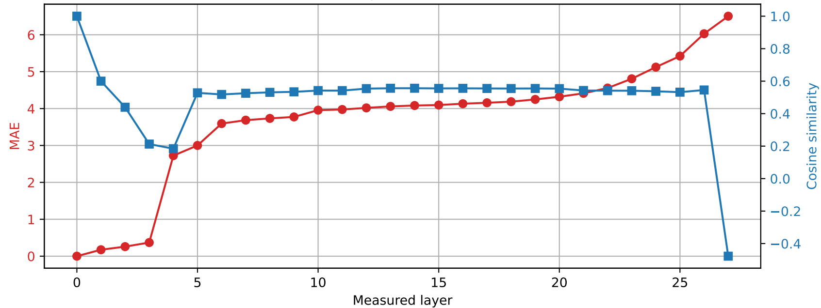
Qwen2.5-7B-Instruct | Prompt 3 Spared layer 9 | Hybrid vs unquantized
