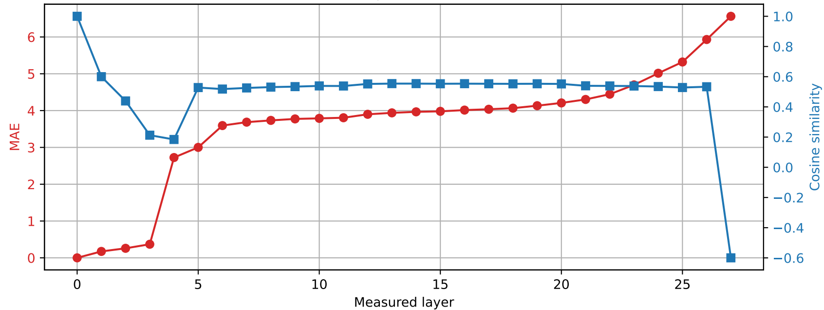
Qwen2.5-7B-Instruct | Prompt 3 Spared layer 11 | Hybrid vs unquantized
