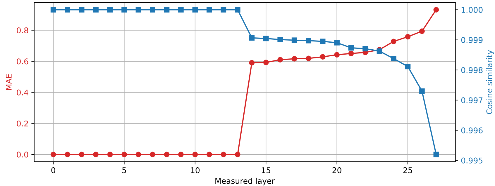
Qwen2.5-7B-Instruct | Prompt 3 Spared layer 13 | Hybrid vs quantized
