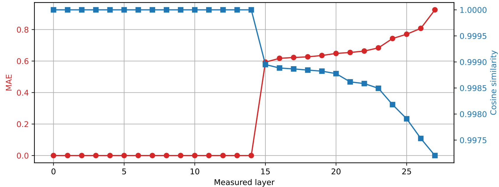
Qwen2.5-7B-Instruct | Prompt 3 Spared layer 14 | Hybrid vs quantized
