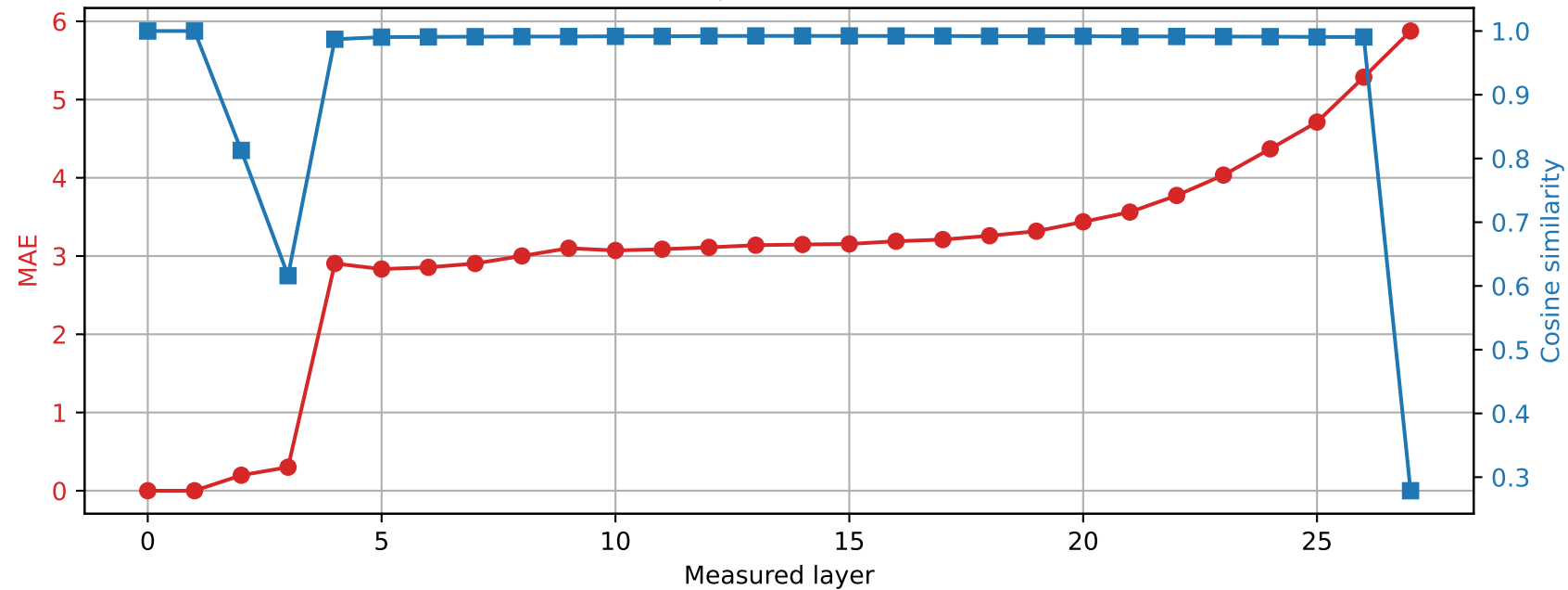
Qwen2.5-7B-Instruct | Prompt 4 Spared layer 0 | Hybrid vs unquantized
