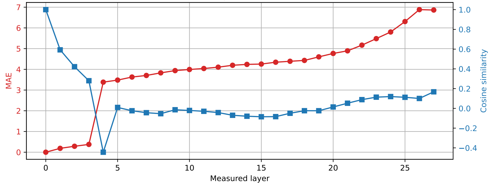
Qwen2.5-7B-Instruct | Prompt 4 Spared layer 24 | Hybrid vs unquantized
