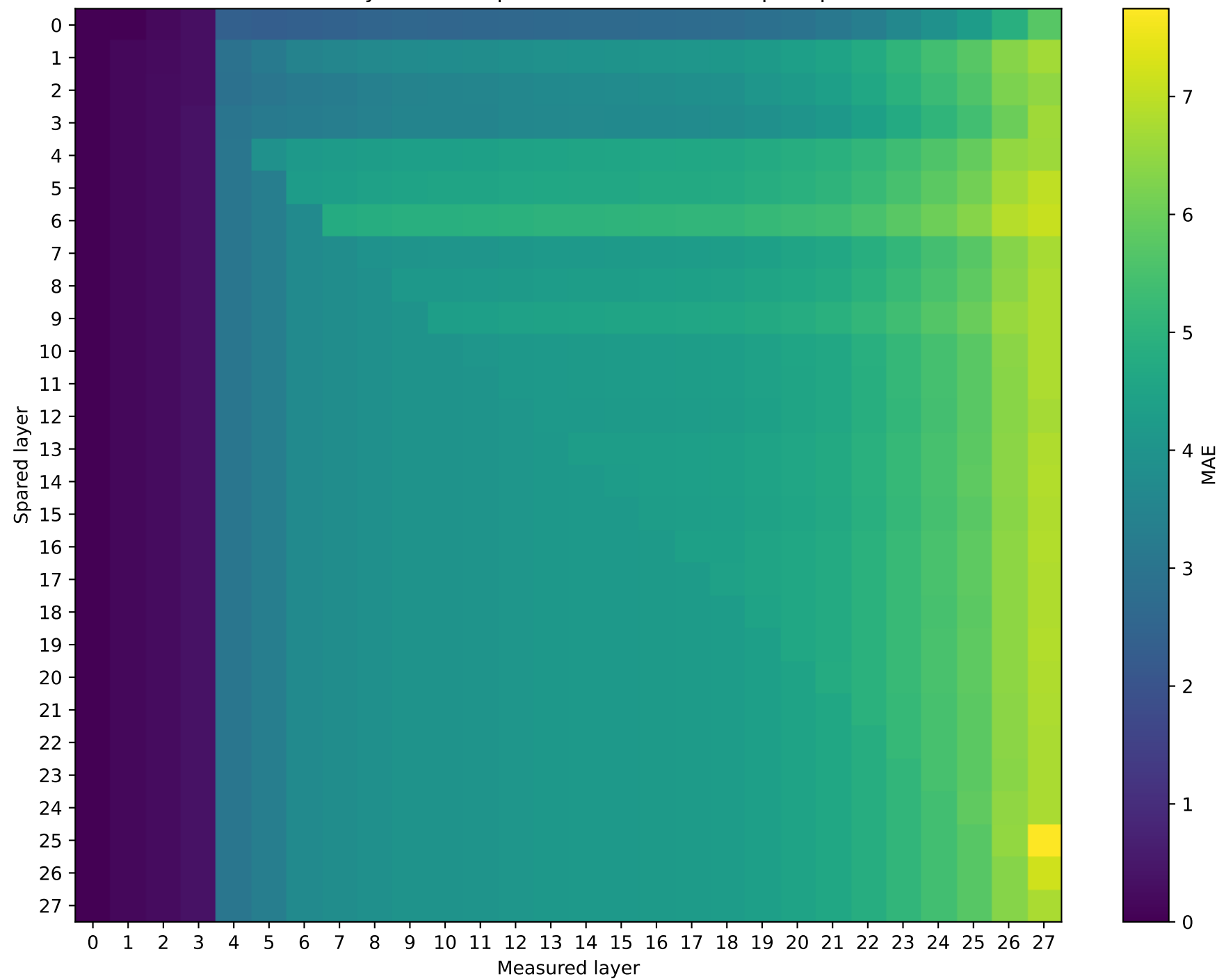
Qwen2.5-7B-Instruct Mean hybrid vs unquantized MAE across 5 prompts
