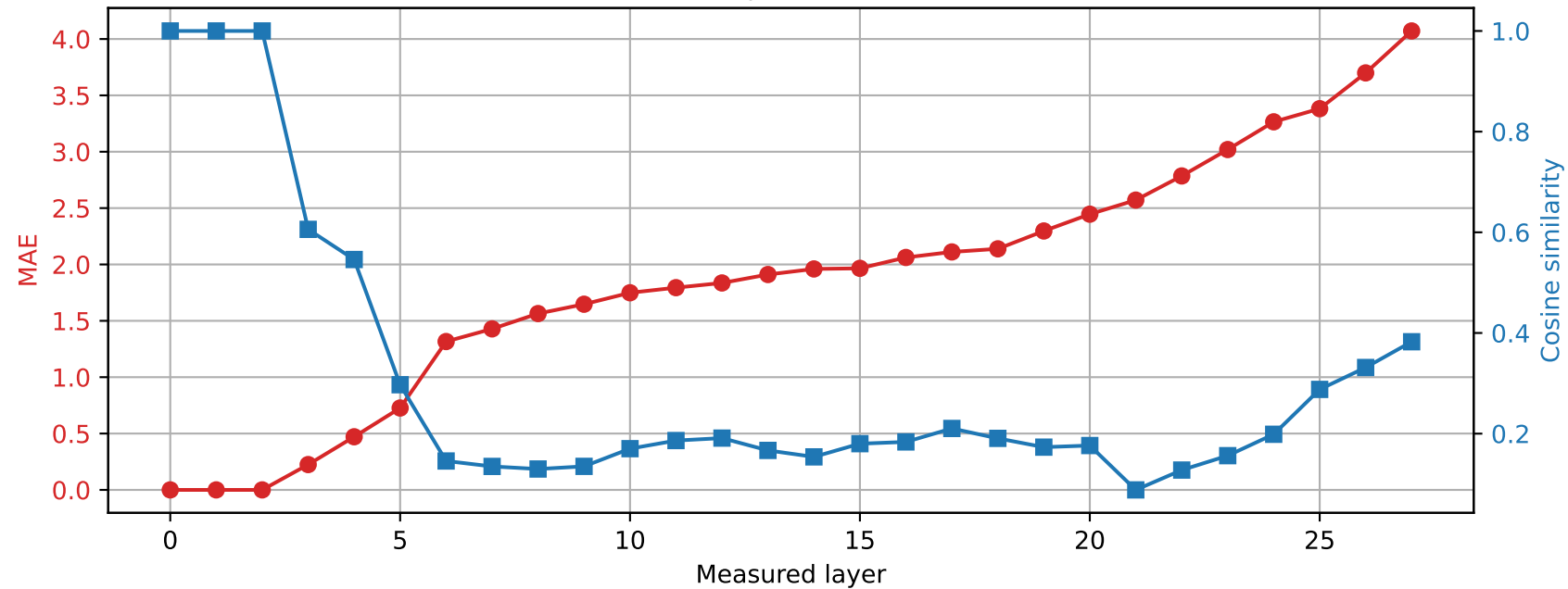
Qwen2.5-7B-Instruct | Prompt 0 Spared layer 2 | Hybrid vs quantized
