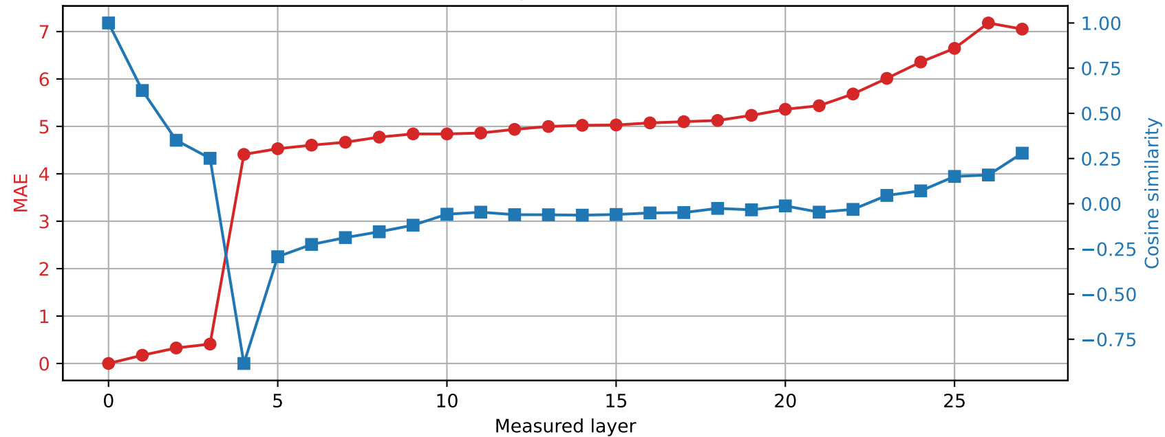
Qwen2.5-7B-Instruct | Prompt 0 Spared layer 3 | Hybrid vs unquantized
