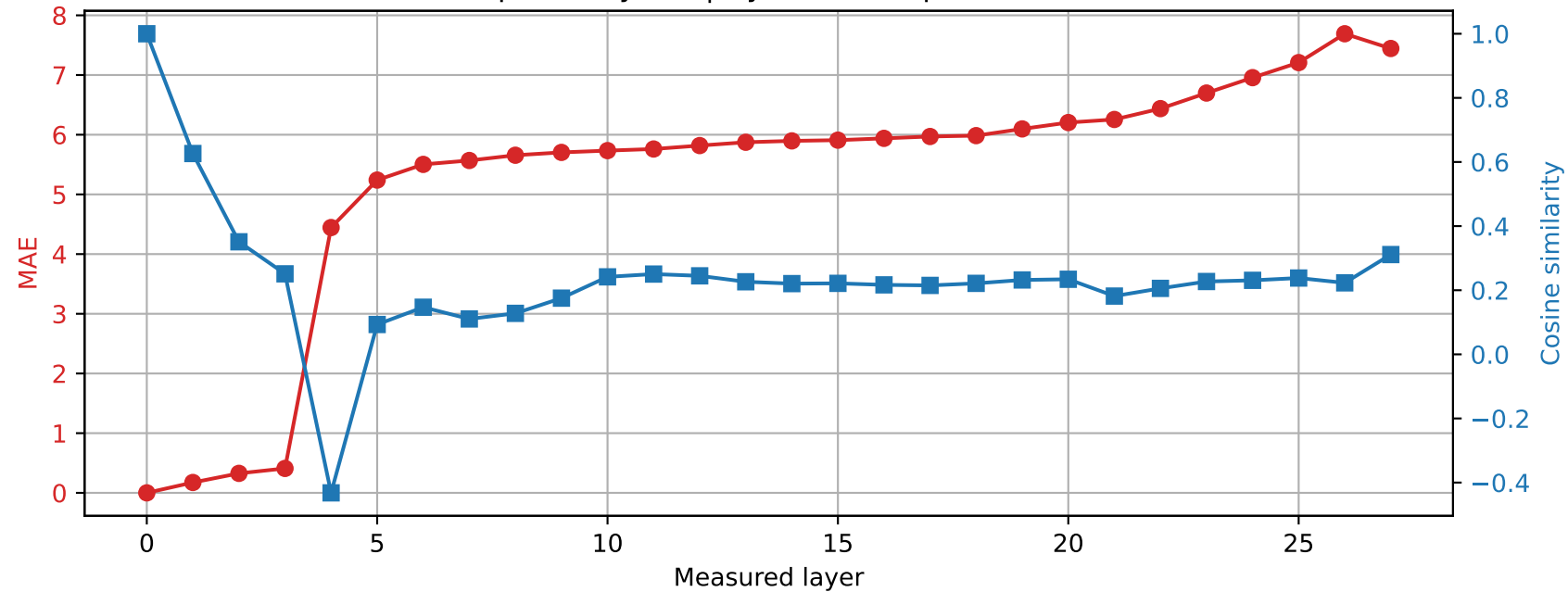
Qwen2.5-7B-Instruct | Prompt 0 Spared layer 4 | Hybrid vs unquantized
